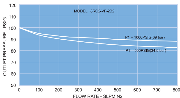
REGULATOR DISCHARGE CHARACTERISTICS CURVES
