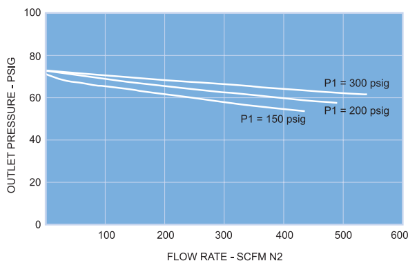
DISCHARGE CHARACTERISTICS CURVES
