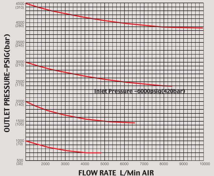
REGULATOR DISCHARGE CHARACTERISTICS CURVES
