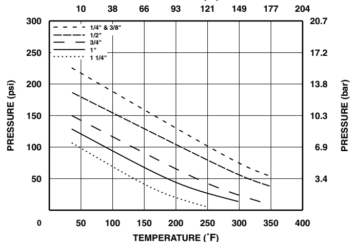
PARFLARE FITTINGS WITH PVDF AND PFA NUTS PRESSURE VS. TEMPERATURE TEMPERATURE (°C)
