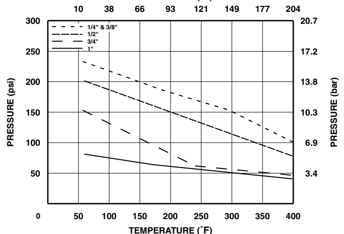
PARFLARE FITTINGS WITH HT NUT ASSEMBLIES PRESSURE VS. TEMPERATURE TEMPERATURE (°C)
