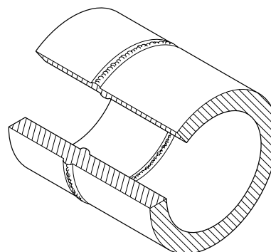
Condition- Bubbles in weld joint. Causes- Overheating of material prior to joining.
