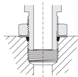
Fig. 4 - Fitting Lock Nut Tightened to Appropriate Torque
