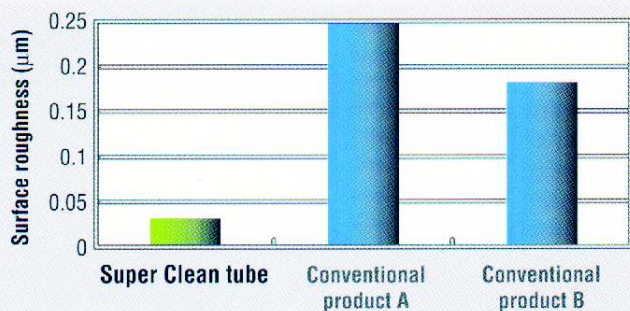
Fig. 1 Measurement result of surface roughness (Ra)
