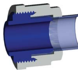
<1/4", 3/8", 1/2", 3/4", 1" Nut>
