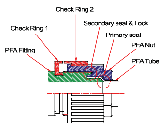
<1/4", 3/8", 1/2", 3/4", 1" Nut>
