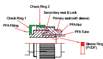
<1/4", 3/8", 1/2", 3/4", 1" Nut>
