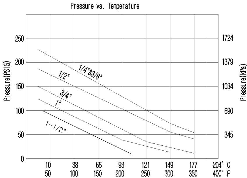
FIG. 1 Pressure rating As a function of temperature. (standard wall th'k)
