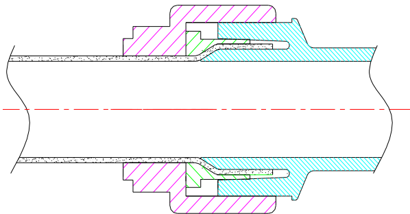
FIG. 3 1-1/2" fitting connection
