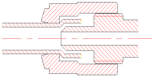
FIG. 2 Eu-Tek Tube fitting connection
