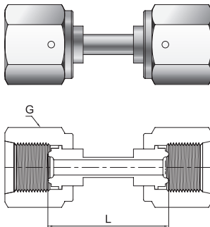
Welded Female Union
