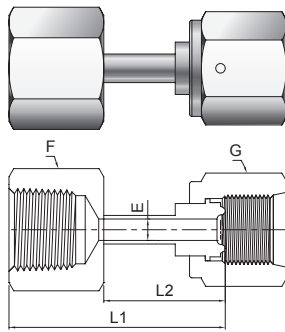
Welded Female Connector (NPT)
