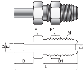
HMFS Bulkhead Connector
