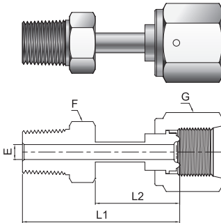
Welded Male Connector (PT)
