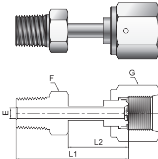
Welded Male Connector (NPT)
