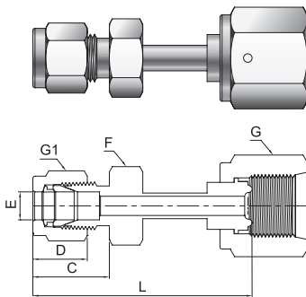
Welded Lok Connector
