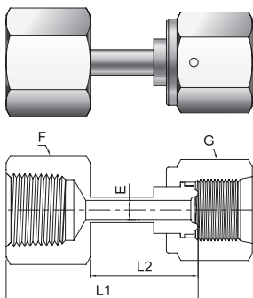
Welded Female Connector (PT)
