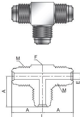
Union Tee
