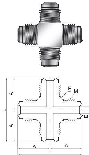
Union Cross
