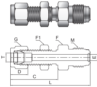
Tube Fitting Bulkhead Connector
