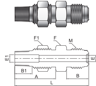
Male Connector (PT)
