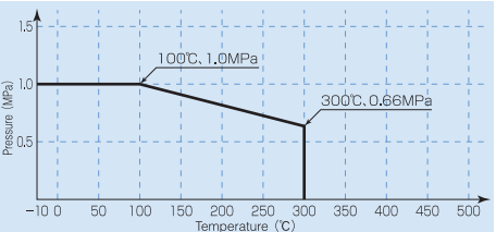
Temperature/Pressure Rating
