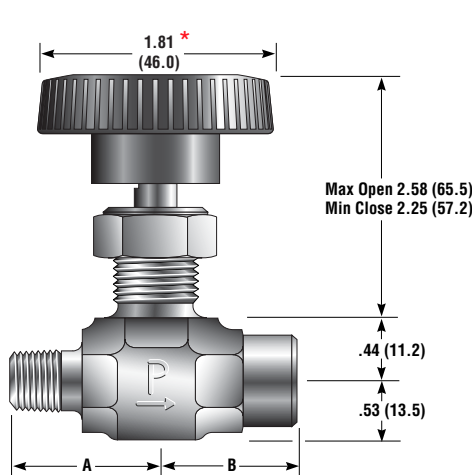
Model Shown: 6M4F-V6LR-V-SS
